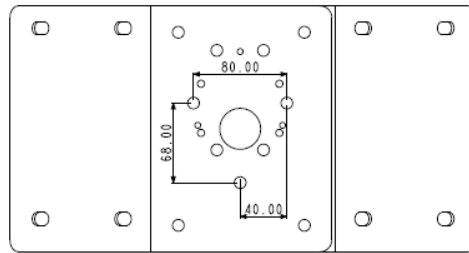
GV-Housing103
