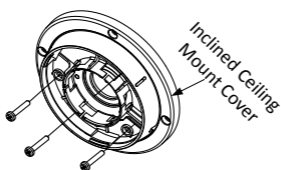
Figure 2-7 Install Turret Camera's Mounting Base
