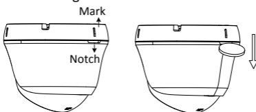
Figure 2-19 Disassemble the Camera
