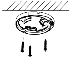
Figure 2-8 Install the Mounting base to Ceiling
