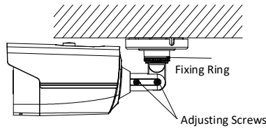
Figure 2-12 Loosen Adjusting Screws and Fixing Ring
