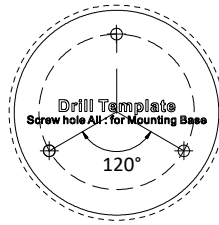
Figure 2-7 Drill Template
