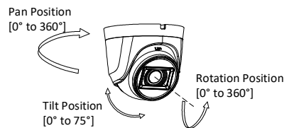
Figure 2-6 3-axis Adjustment
