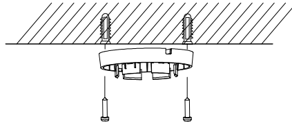
Figure 2-4 Install the Mounting Base to Cement Ceiling
