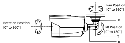
Figure 2-13 3-Axis Adjustment
