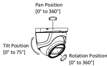
Figure 2-9 3-Axis Adjustment
