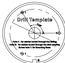
Figure 2-2 Drill Template
