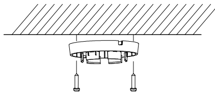
Figure 2-3 Install the Mounting Base to Wooden Ceiling
