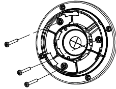
Figure 2-6 Install Turret Camera's Mounting Base
