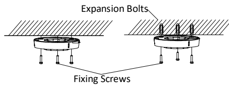
Figure 2-2 Attach the Mounting Base to the Ceiling
